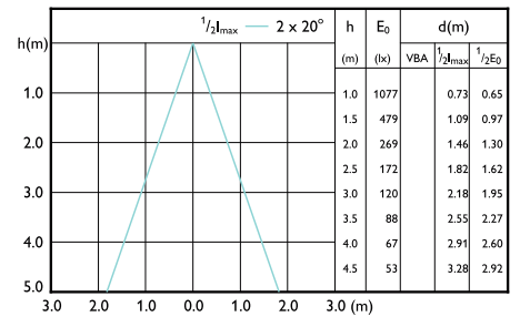
LEDspot MAS VLE 7-50W GU5.3 MR16 840 36D DIM
