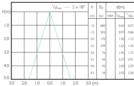
CorePro LEDspotLV 35W GU5-3 840 36D
